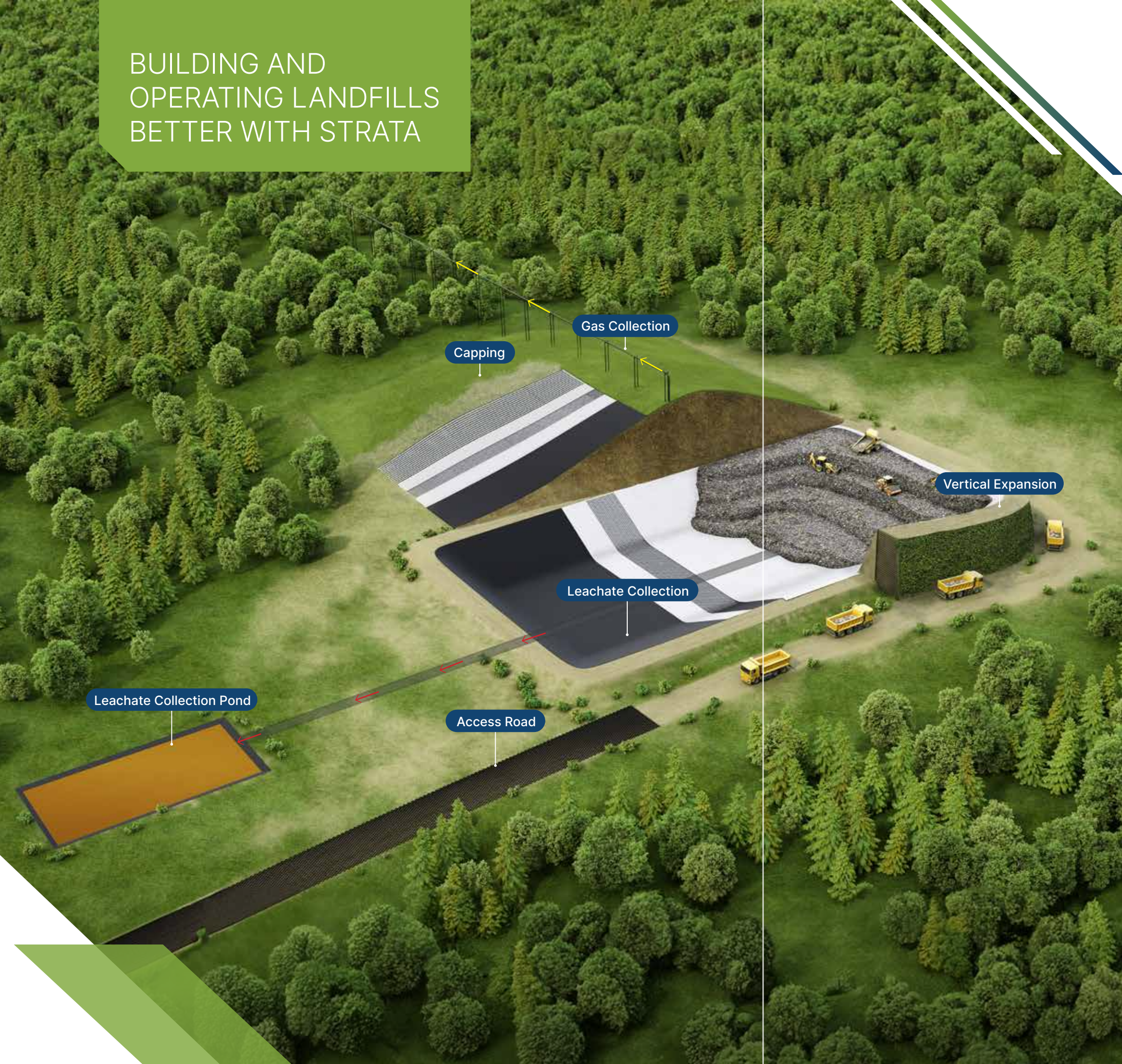
« Capping Drainage, Veneer Stability, Erosion Control
