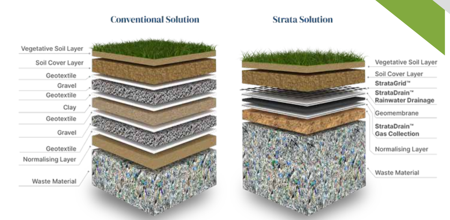
Veneer: Conventional Vs Strata Solution
