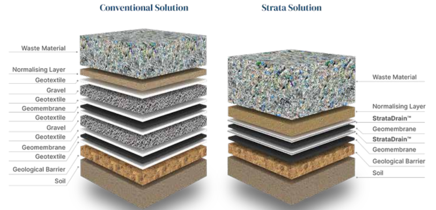
Leachate Collection and Leak Detection: Conventional Vs Strata Solution
