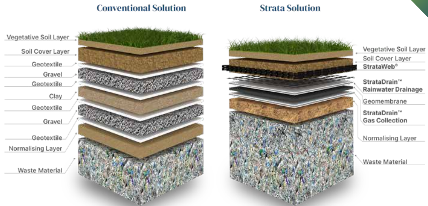
Erosion Control: Conventional Vs Strata Solution
