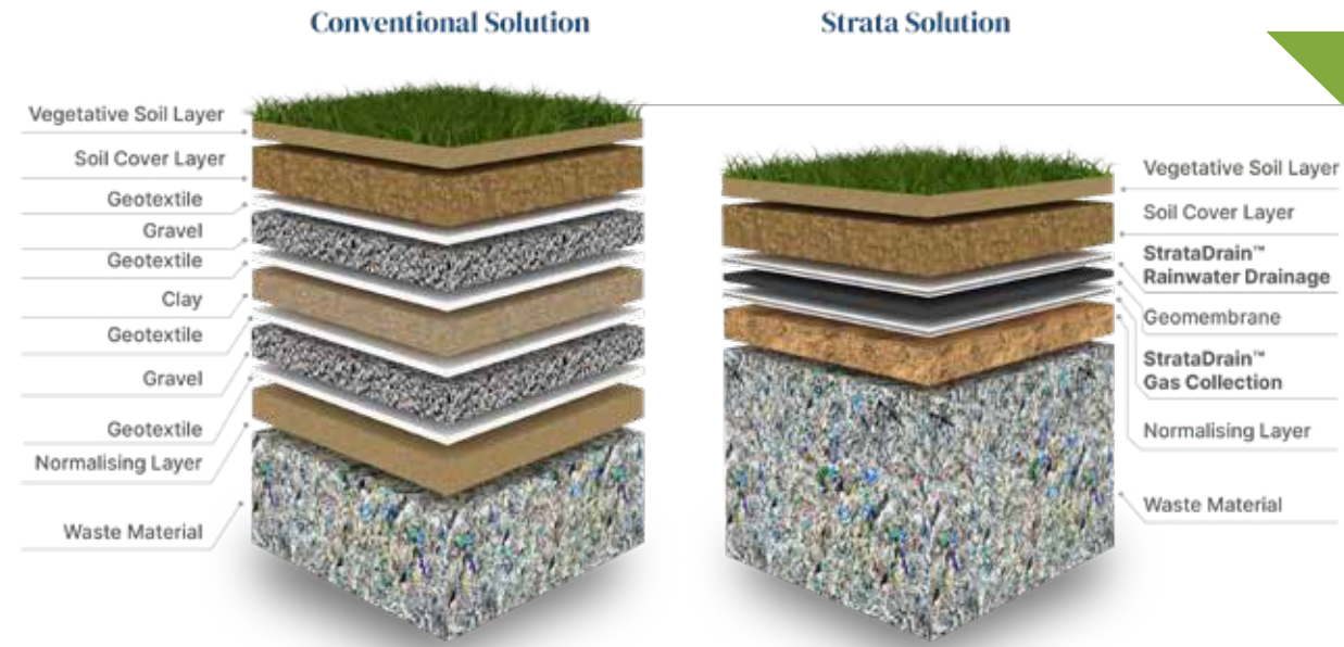
Capping System: Conventional Vs Strata Solution
